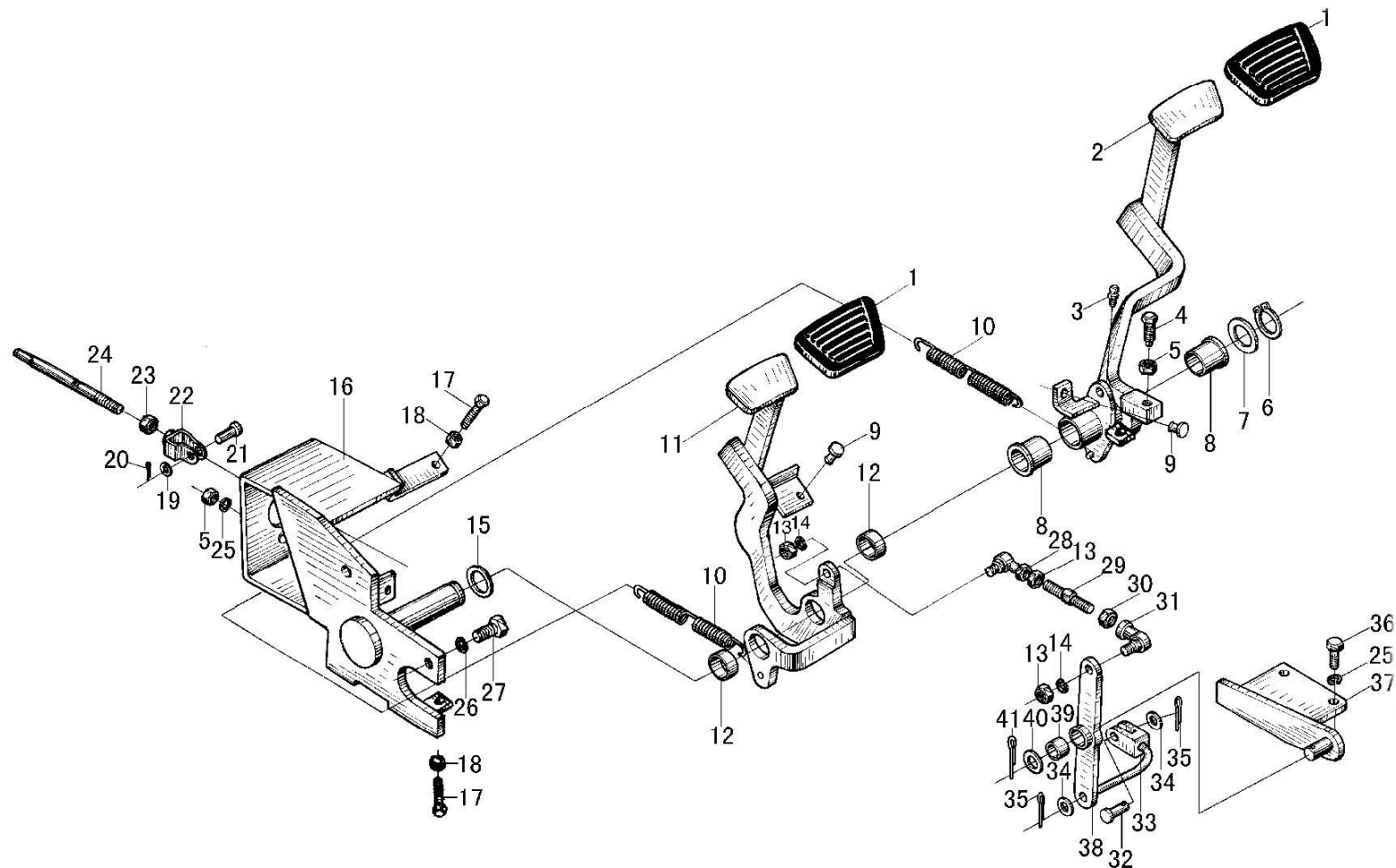
Fig. 2 Brake and inch pedal assy
