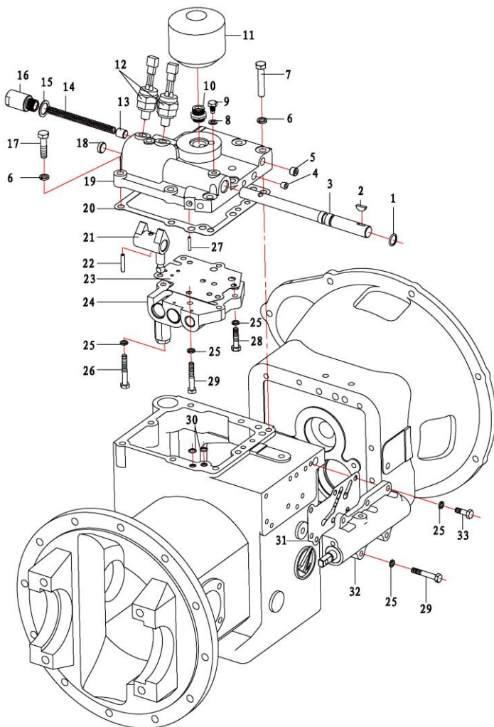
图 29 盖、控制阀、微动阀（液力式）中南 Fig.29 Cover control valve & inching valve (tor-con type) ZhongNan
