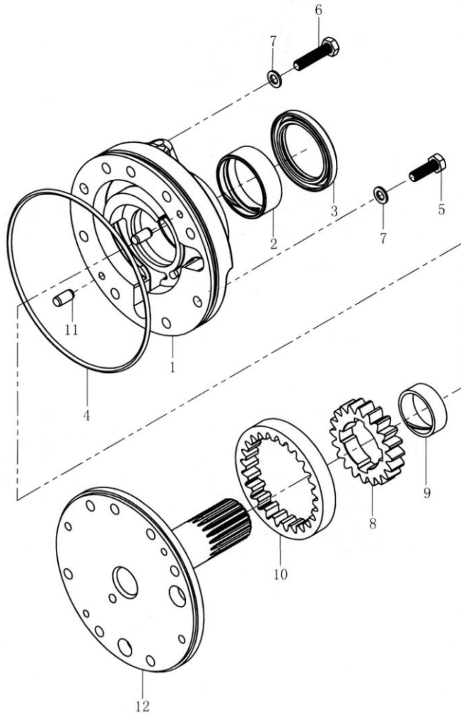
图 23 供油泵（液力式）绍兴 SHAOXIN Fig.23 Charging pump(tor-con type)
