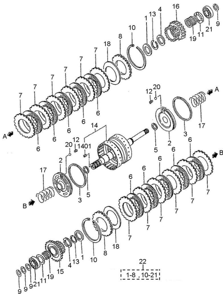
图 34 变速箱 (其 2) Fig.34 Transmission (part-2)
