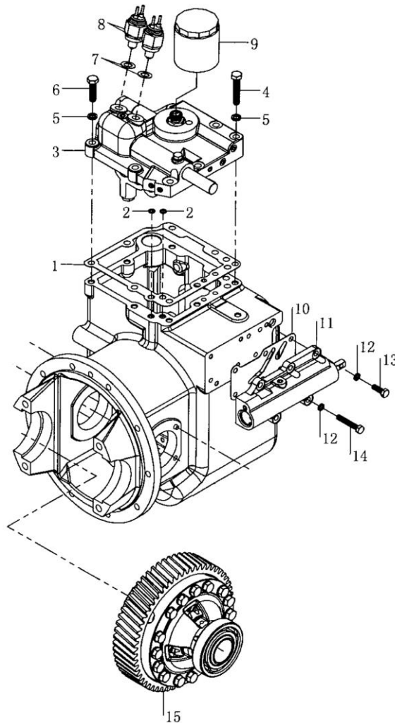
图 21 盖、控制阀、微动阀（液力式）绍兴 Fig.21 Cover control valve & inching valve (tor-con type) SHAOXIN
