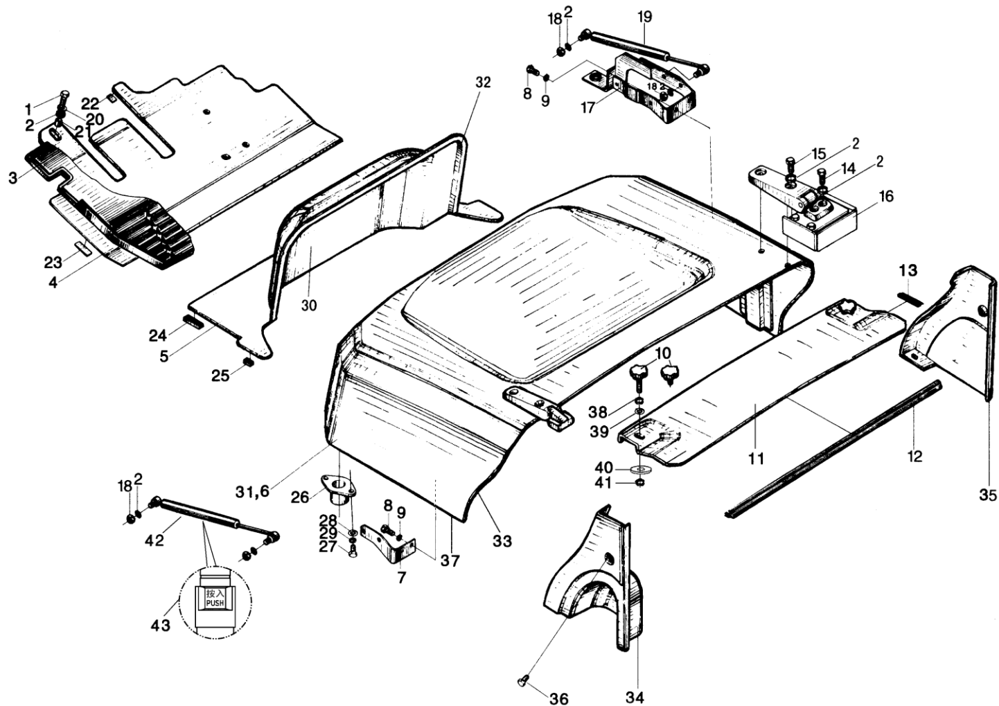
图 6 机罩及底板总成(I) Fig.6 Hood and floor board assy( I )
